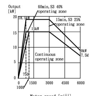
MODEL \beta iP 30/6000
