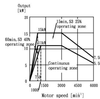
MODEL \beta iP 22/6000
