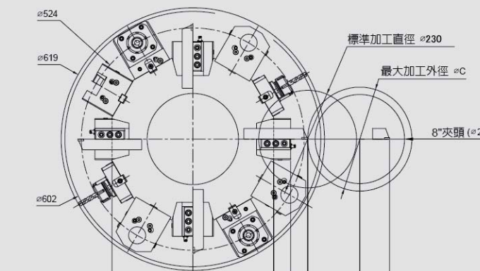
(12T)BMT65-380
