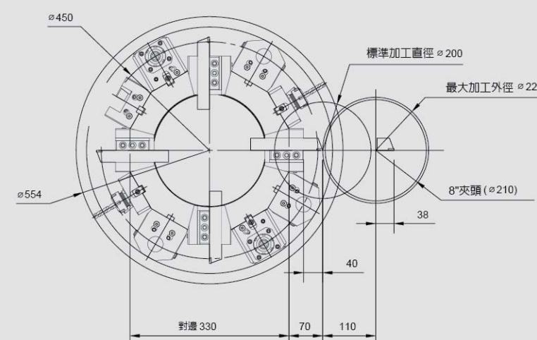
FTC-15MY Tool Interference
