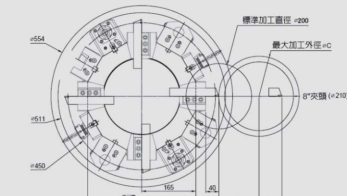
(12T)BMT55-330
