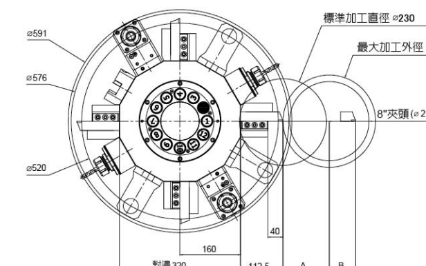
(12T)VDI40-320
