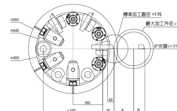
(12T)VDI-40-PCD370
