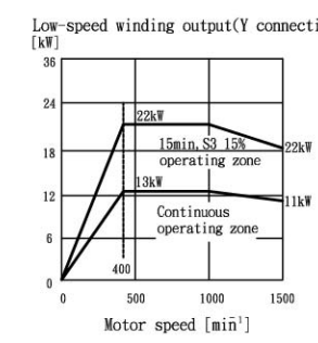
MODEL \alpha 40/6000rP
