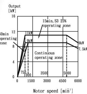
MODEL \beta iP 18/6000
